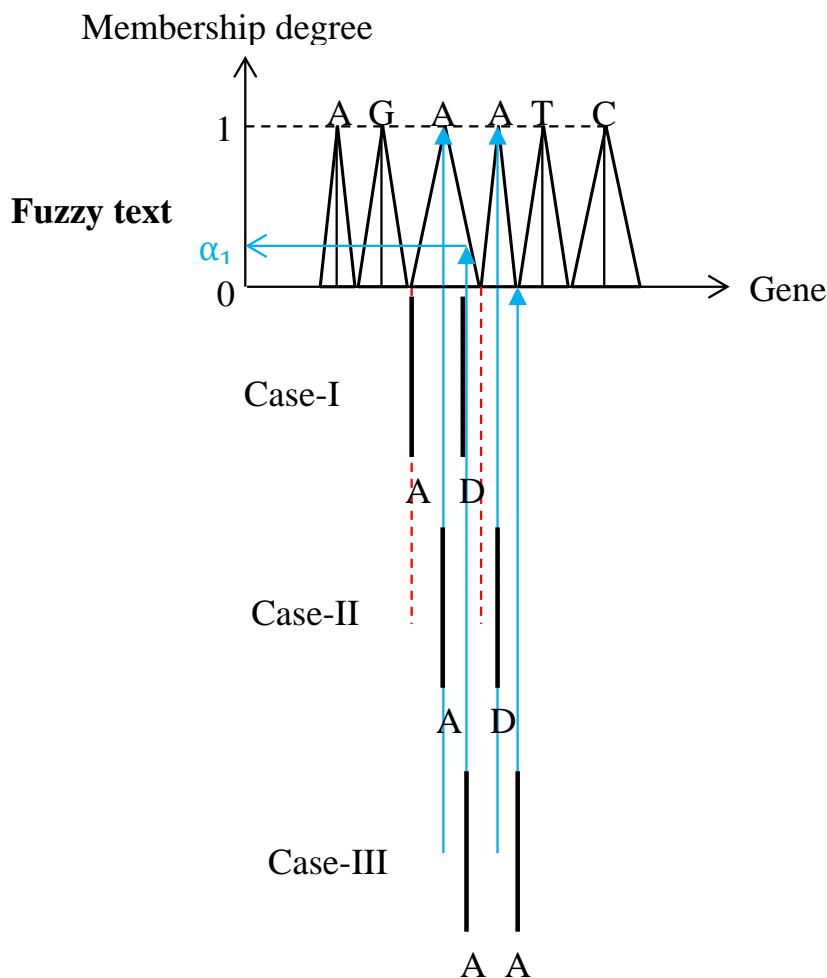
Fig. (7). Naive strand match algorithm with fuzzy text and crisp pattern.
