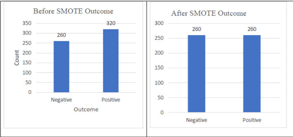
Fig. (2). SMOTE Outcome: Before and after.
